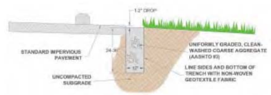
FILTER STRIP WITH GRAVEL TRENCH LEVEL SPREADER
