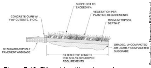
FILTER STRIP WITH CURB OPENING
