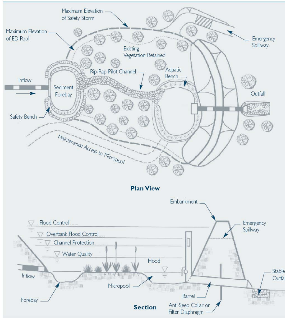
Figure 7.20: Extended detention basin schematic
