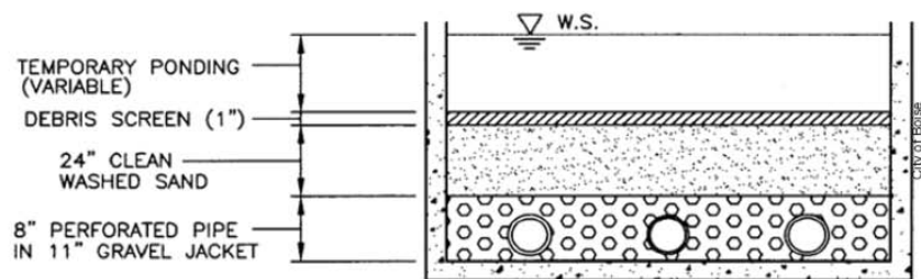
PROFILE
