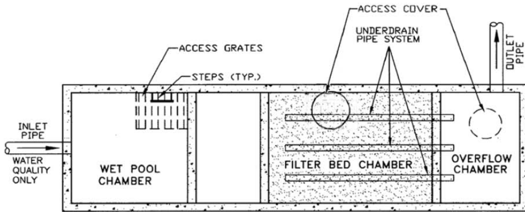
PLAN VIEW
